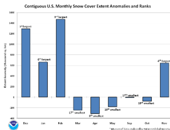
U.S. Monthly Snow Cover Extent Anomalies Data Source: Rutgers Global Snow Lab
