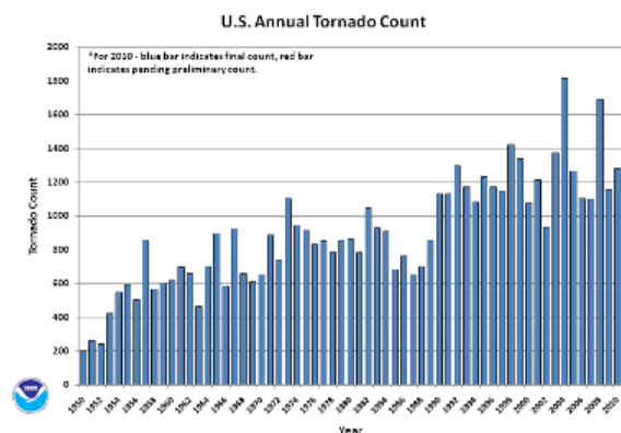
Annual Tornado Counts 1950-2010
