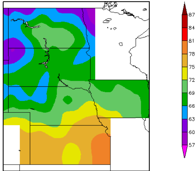
Figure 1: Soil temperature (°F) at 4 inches (10 cm) depth for June 9, 2010. Maps are also available for a one-week time interval.
