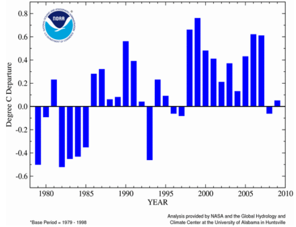
Jan-Dec Lower Tropospheric Temperature Anomalies Contiguous U.S., 1979-2009
